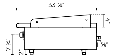
COMMON SIDE VIEW
